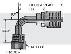
Komatsu Style Swivel Female Stem 90° Seat
