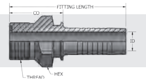
Solid Male Flat Face O-Ring Seal Stem
