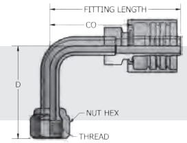
JIC 37° Swivel Female Stem 90° Bent Tube Medium Drop
