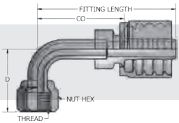
JIC 37° Swivel Female Stem 90° Bent Tube Short Drop
