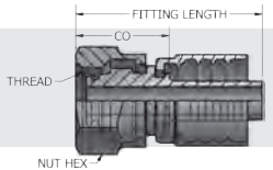
Metric Swivel Female Stem DIN 20078 Heavy Straight with O-Ring and 12/30° Univ. Cone
