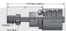
SAE 45° Male Inverted Swivel Stem Straight Tube
