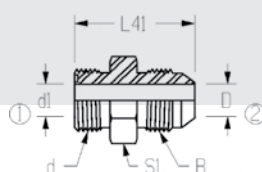
FF7403 37° Male JIC/Male ORFS Adapter
