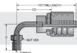
SAE 45° Male Inverted Swivel Stem 90° Bent Tube
