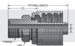
Solid Male Flat Face O-Ring Seal Stem
