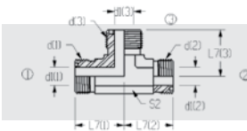
FF2603 Union Tee
