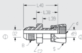
FF7504 37° Male JIC/Female ORFS Swivel Adapter
