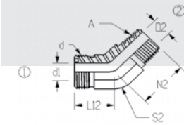
FF2503 45° Male Elbow
