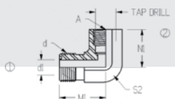
FF2502 90° Female Elbow
