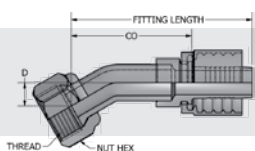
JIC 37° Swivel Female Stem 30° Bent Tube Short Drop
