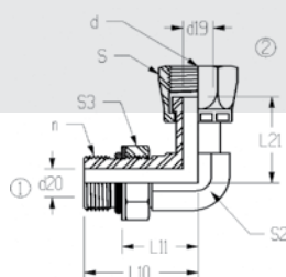
FF6809 90° Straight Thread/Female ORFS Swivel Elbow
