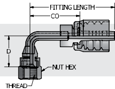
JIC 37° Swivel Female Stem 90° Bent Tube Short Drop Crimp Style
