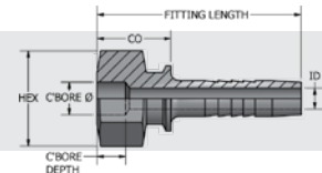
Tube Stem Flat Face O-Ring Seal
