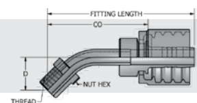
SAE 45° Male Inverted Swivel Stem 45° Bent Tube
