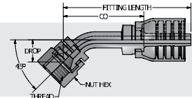
Komatsu Style Swivel Female Stem 45° Seat
